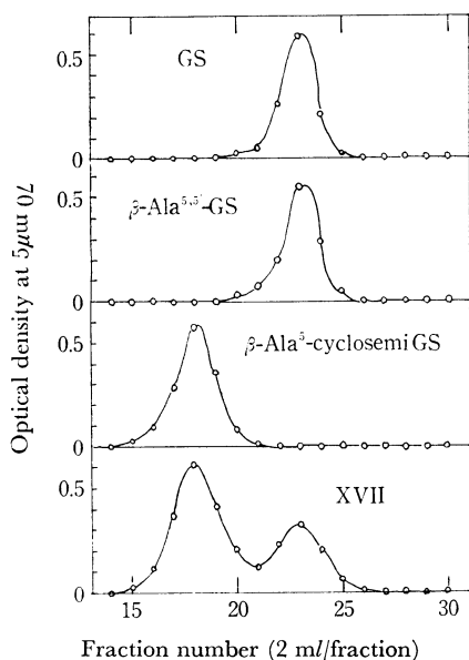
Fig. 4. Carboxymethylcellulose column chromatography of the compounds.
